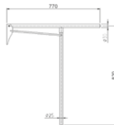
Asidero abatible 180°con pata Folding support rail with leg
