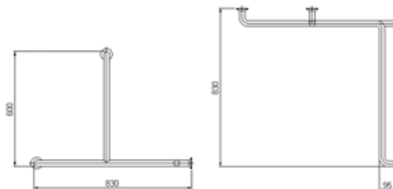
Asidero 90°escuadra horizontal 90° grab rail squarely
