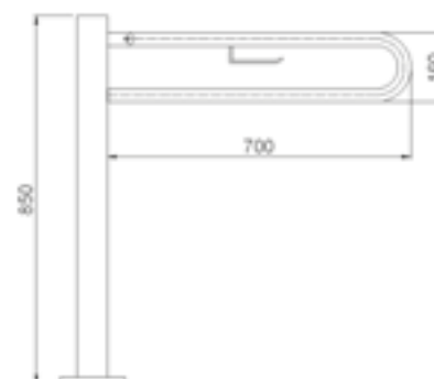
Asidero abatible 180°con pedestal 180° floor mounted folding support rail
