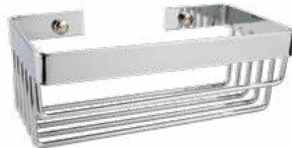
130601-AR Esponjera rectangular Square shower basket DIM: 200 mm. x 100 mm. x 75 mm.
