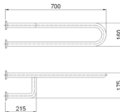
Asidero fijo 180°/180° wall mounted grab rail
