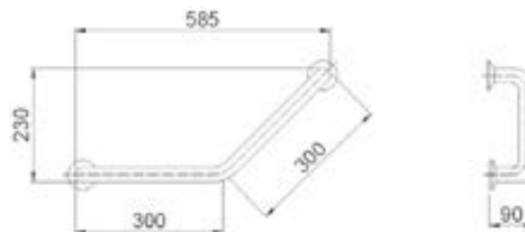
Asidero 45°45° angled grab rail
