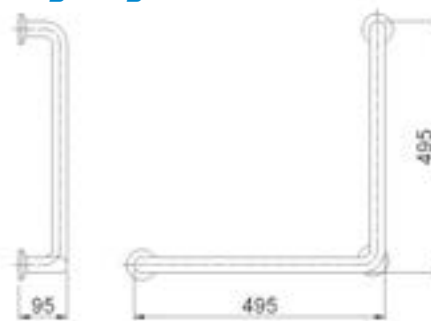
Asidero 90°90° angled grab rail
